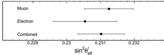
CMS Nominal NNPDF3.0 18.8 ( \mu\mu ) + 19.6 (ee) \text{fb}^{-1} (8 TeV)
