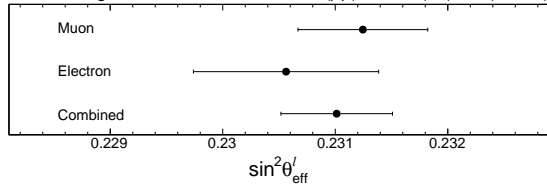
CMS Weighted NNPDF3.0 18.8 ( \mu\mu ) + 19.6 (ee) \text{fb}^{-1} (8 TeV)
