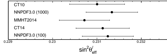
CMS Weighted PDF 18.8 fb -1 (8 TeV)
