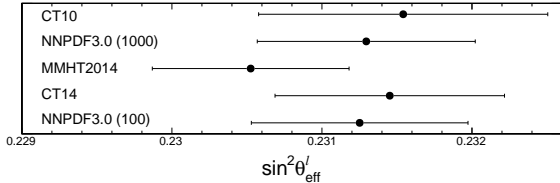
CMS Nominal PDF 18.8 fb -1 (8 TeV)
