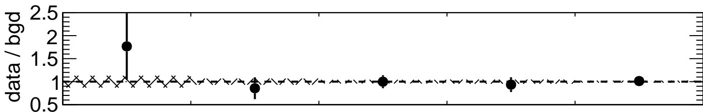
Lost-lepton and three-lepton background control regions
