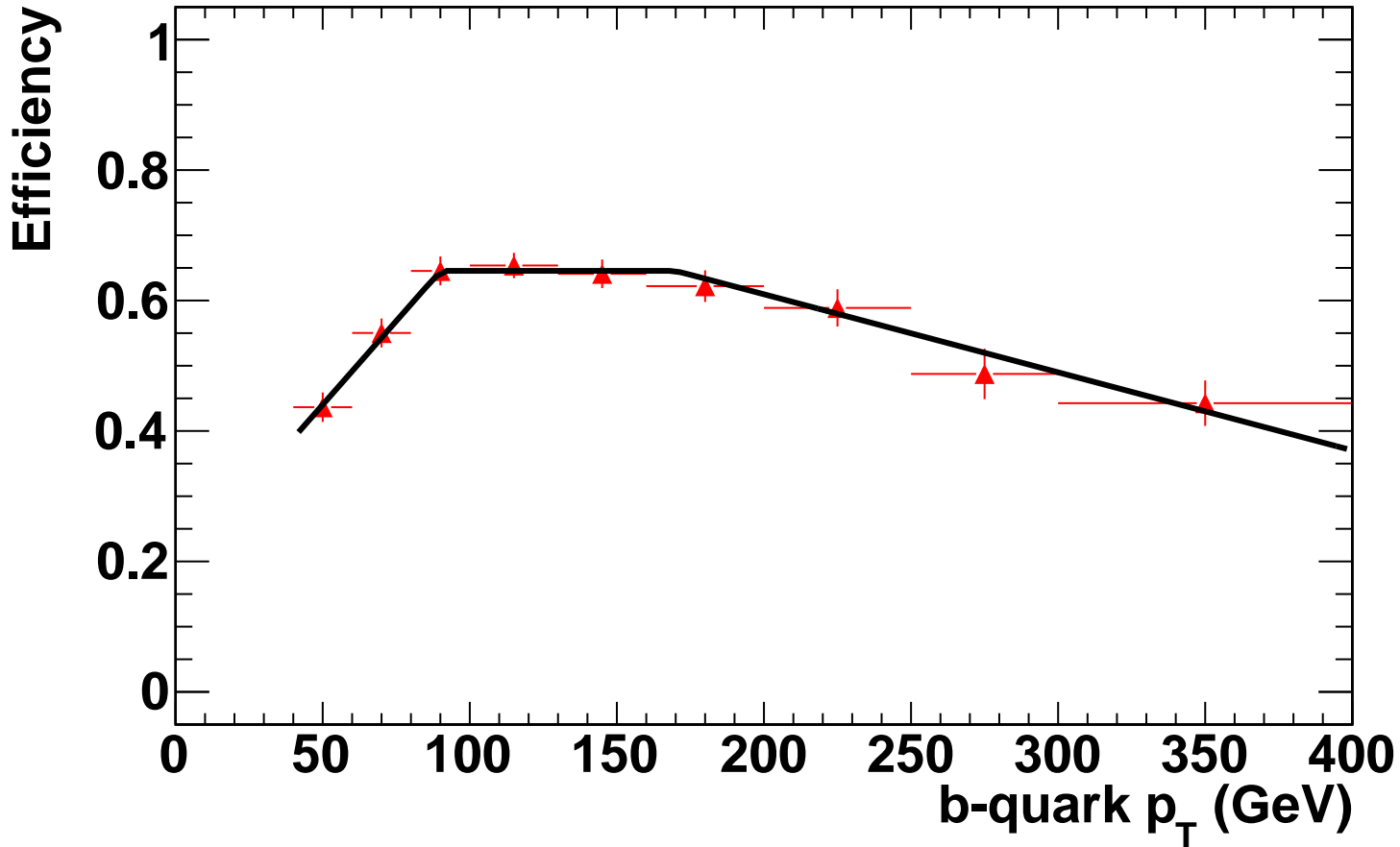
CMS Simulation, \sqrt{s} = 7 TeV
