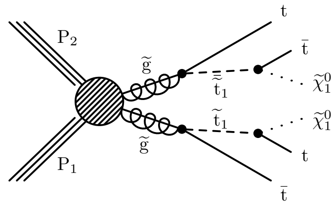
(c) T5tttt
