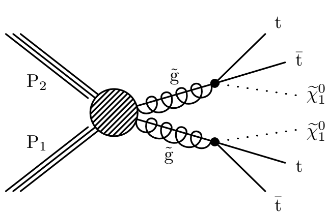
(a) T1tttt
