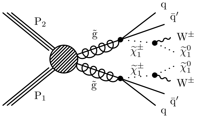
(e) T5qqqqWW
