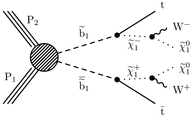
(f) T6ttWW
