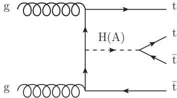
(a) t\bar{t}H
