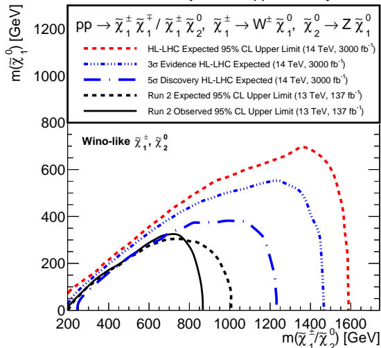
CMS Phase-2 Projection Supplementary
