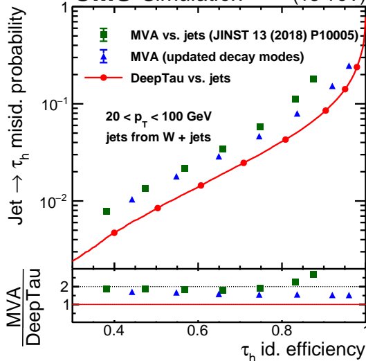
CMS Simulation (13 TeV)
