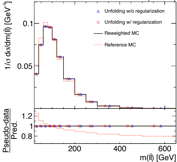
CMS Simulation 138 \text{ fb}^{-1} (13 TeV)
