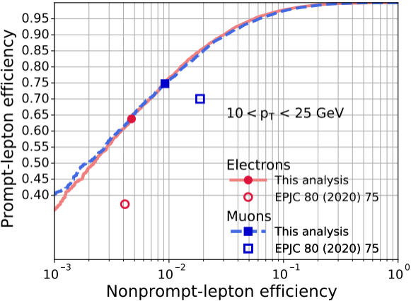
CMS Simulation (13 TeV)
