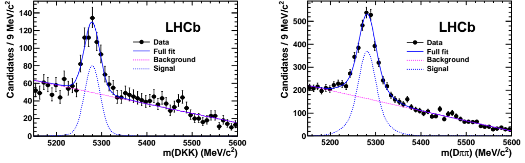
Figure 1: Fit to the B candidate invariant mass distribution for events in the D sidebands for the (left) \bar{D}^0 K^+ K^- and (right) \bar{D}^0 \pi^+ \pi^- decay mode. The data points are shown in black with the components of the fit overlaid; full fit (solid blue), double Gaussian signal (dashed blue) and linear background (dashed pink).
