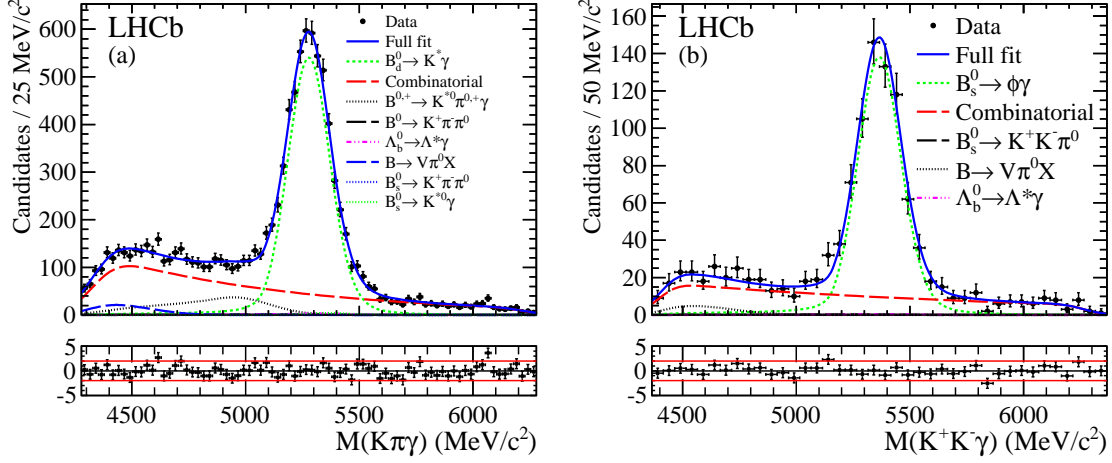
Figure 1: Simultaneous fit of the full 2011 data for (a) B^0 \rightarrow K^{*0}\gamma and (b) B_s^0 \rightarrow \phi\gamma candidates. The black points represent the data and the fit result is represented as a solid blue line. The various background components are also displayed. The Poisson \chi^2 residuals, described in Ref. [22] of the main paper, are shown below the fits with the \pm 2\sigma confidence-level interval delimited by solid red lines.
