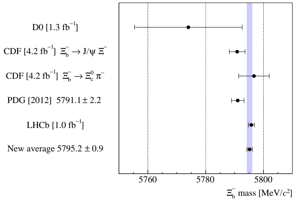
Figure 2: Measurements of the \Xi_b^- mass. The new average is performed using the PDG prescription.
