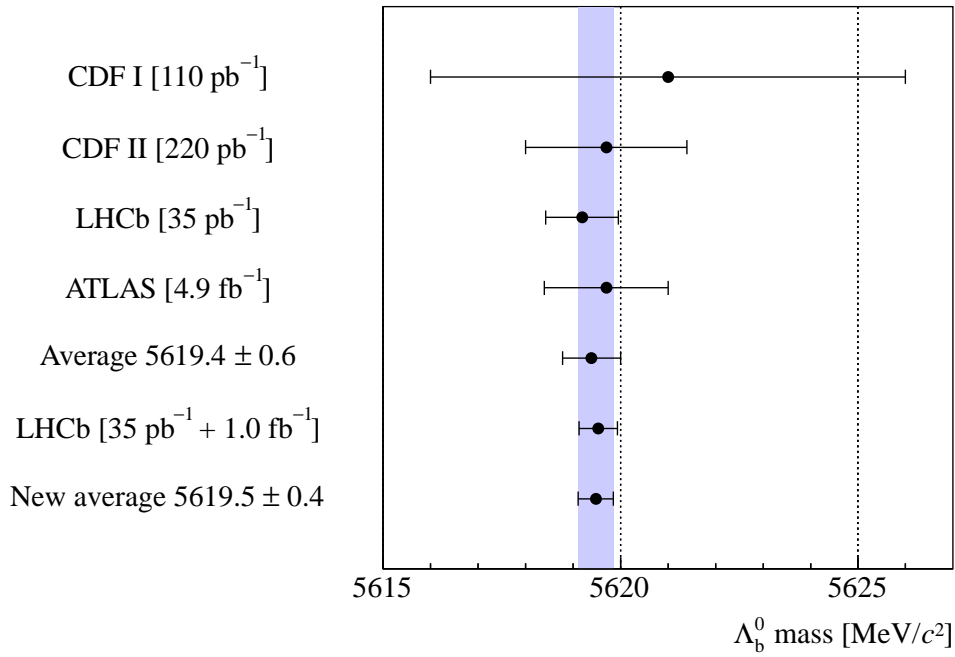
Figure 1: Measurements of the \Lambda_b^0 mass. The new average is performed using the PDG prescription.
