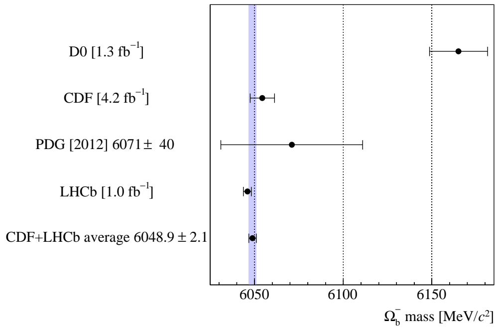
Figure 3: Measurements of the \Omega_b^- mass. The CDF + LHCb average is performed using the PDG prescription.
