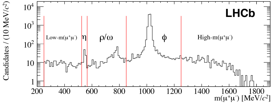
Figure 6: m(\mu^+ \mu^-) spectrum of D_{(s)}^+ \rightarrow \pi^+ \mu^+ \mu^- candidates that pass the final selection and are within 3\sigma of either of the mean values of the Gaussian-like peaks describing the D^+ and D_s^+ signals.
