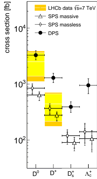
Figure 1: Graphical comparison to theory predictions. The D_s^+ and \Lambda_c^+ states were searched for in the decay channels D_s^+ \rightarrow \phi(\rightarrow K^+K^-)\pi^+ and \Lambda_c^+ \rightarrow pK^-\pi^+ with no observed candidates. The measured cross-section is expected to be the sum of SPS and DPS.
