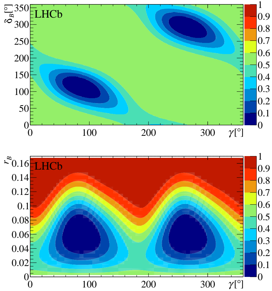
Figure 1: Colour versions of Fig. 7: projections of the p-value regions onto the (\gamma, \delta_B) and (\gamma, r_B) planes with all sources of uncertainty taken into account.
