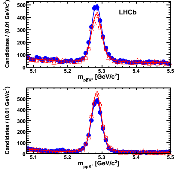
Figure 1: Invariant mass distributions of p\bar{p}K^\pm candidates for m_{p\bar{p}} < 2.85 \text{ GeV}/c^2 , regions (bottom) m_{Kp}^2 < 10 \text{ GeV}^2/c^4 and (top) m_{Kp}^2 > 10 \text{ GeV}^2/c^4 . The blue curve and points with error bars represent negatively-charged p\bar{p}K^- candidates. The red curve and triangles with error bars represent positively-charged p\bar{p}K^+ candidates.
