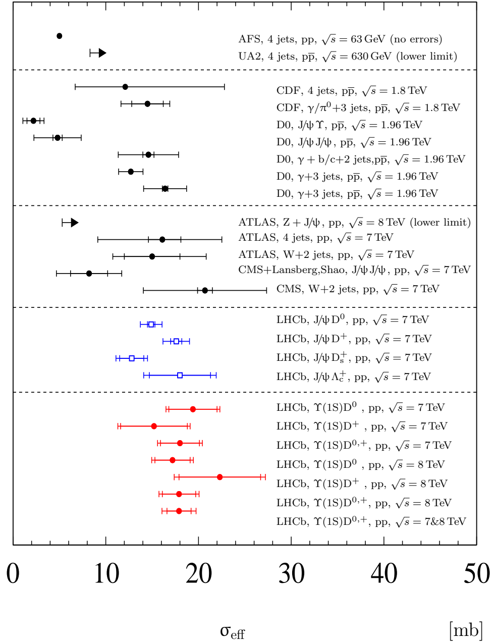
Figure 1: Summary of recent measurements of the effective DPS cross-section \sigma_{\text{eff}} [1–16] When two error bars are shown, the inner error bars indicate the statistical uncertainty whilst the outer error bars indicate the sum in quadrature of the statistical and systematic uncertainties.
