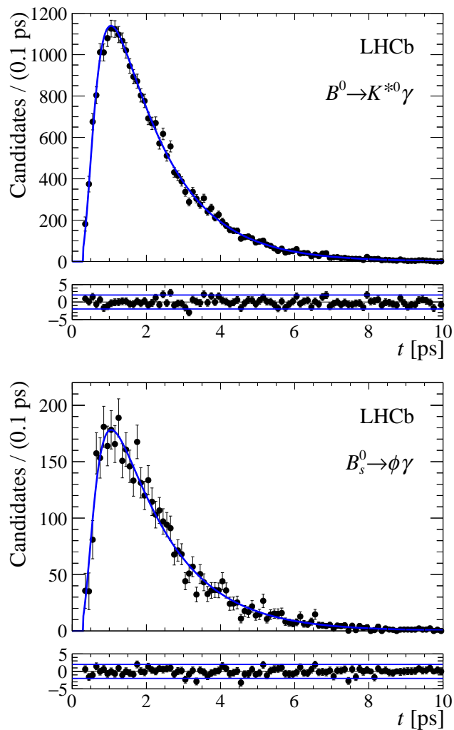
Figure 4: Background-subtracted decay-time distributions for (top) B^0 \rightarrow K^{*0} \gamma and (bottom) B_s^0 \rightarrow \phi \gamma decays with the fit projections overlaid and normalized residuals shown below ( same information as Fig. 2 but with constant binning and linear scale ).
