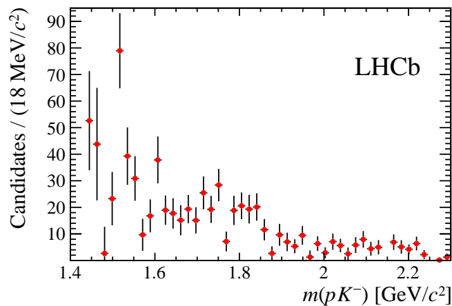
Figure 1: Background-subtracted and efficiency-corrected m(pK^-) distribution for the decay \Lambda_b^0 \rightarrow pK^- \mu^+ \mu^- .
