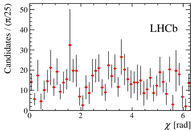
Figure 2: Background-subtracted and efficiency-corrected distribution of the angle \chi for the decay \Lambda_b^0 \rightarrow pK^- \mu^+ \mu^- .
