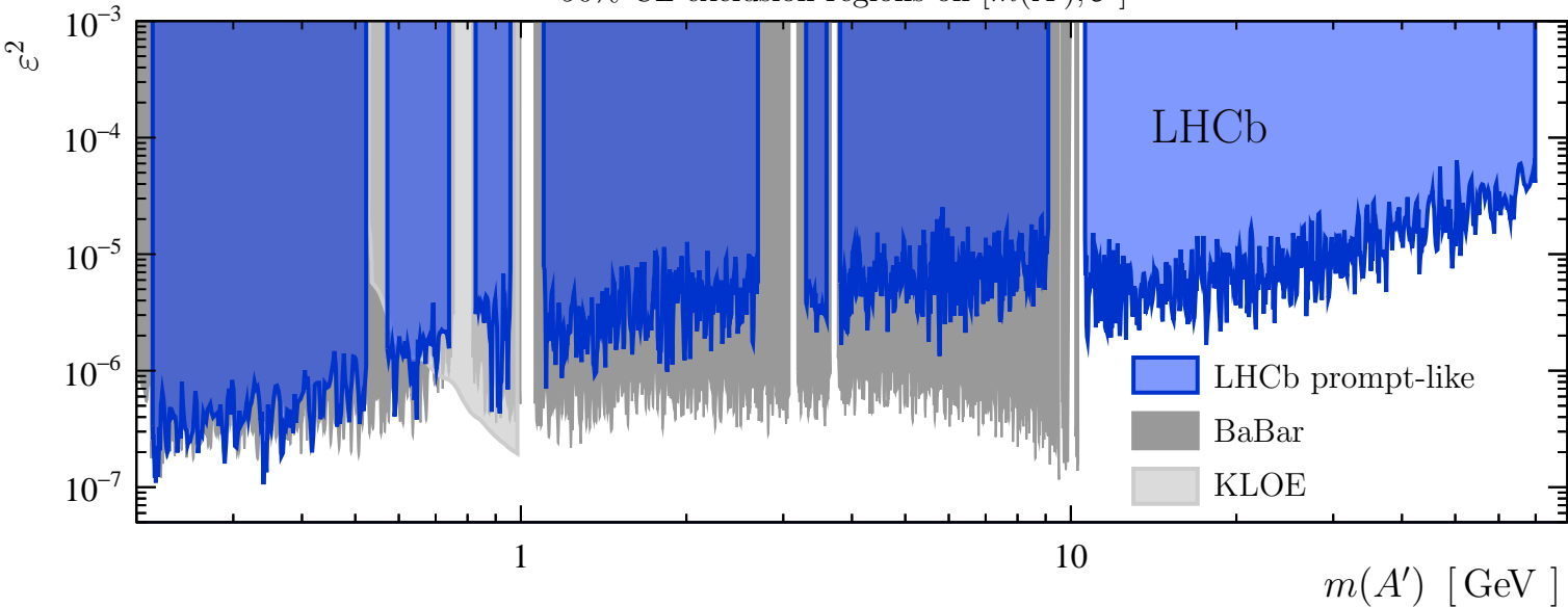
90% CL exclusion regions on [m(A'), \varepsilon^2]
