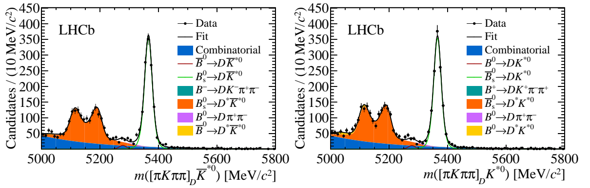
Figure 3: Invariant-mass distributions (data points with error bars) and results of the fit (lines and coloured areas) for (left) \bar{B}^0 \rightarrow D(\pi^- K^+ \pi^+ \pi^-) \bar{K}^{*0} and (right) B^0 \rightarrow D(\pi^+ K^- \pi^+ \pi^-) K^{*0} , shown on a linear scale.
