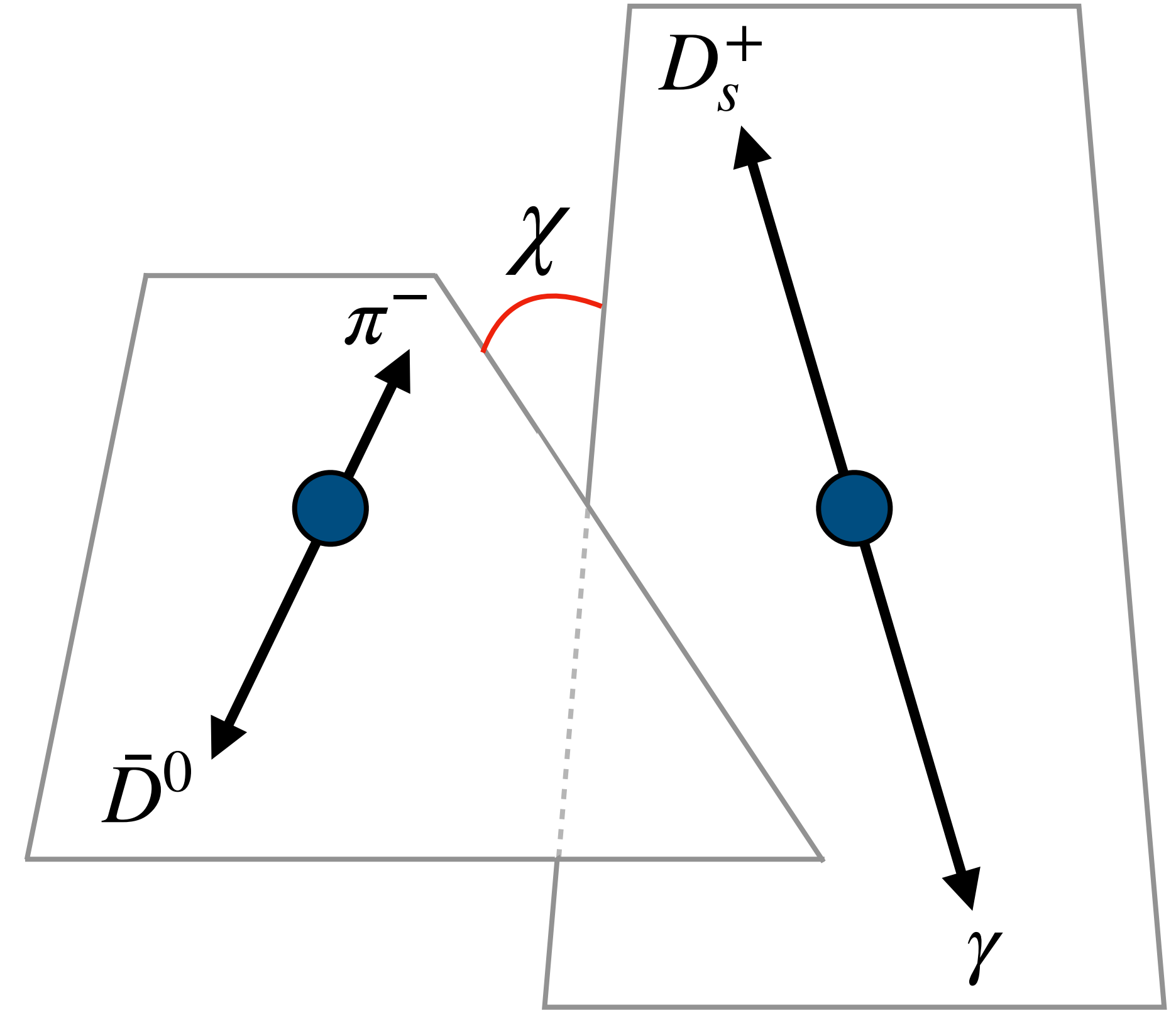
B^0 rest frame
