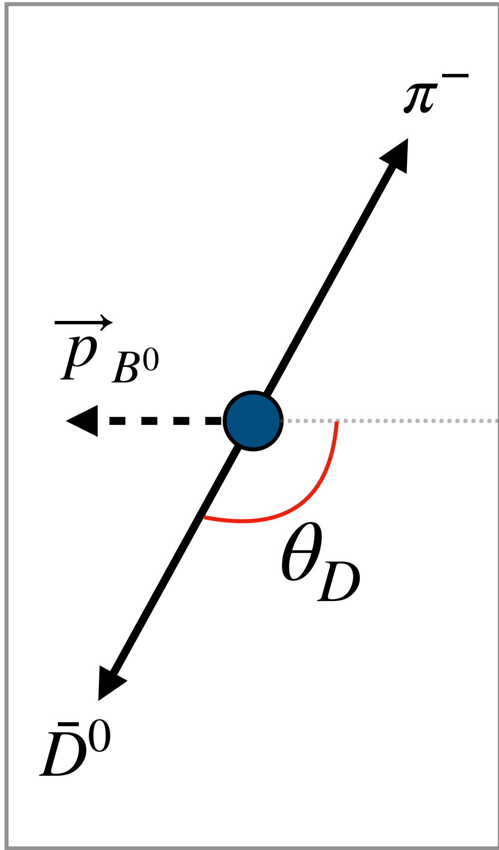
D^{*-} rest frame
