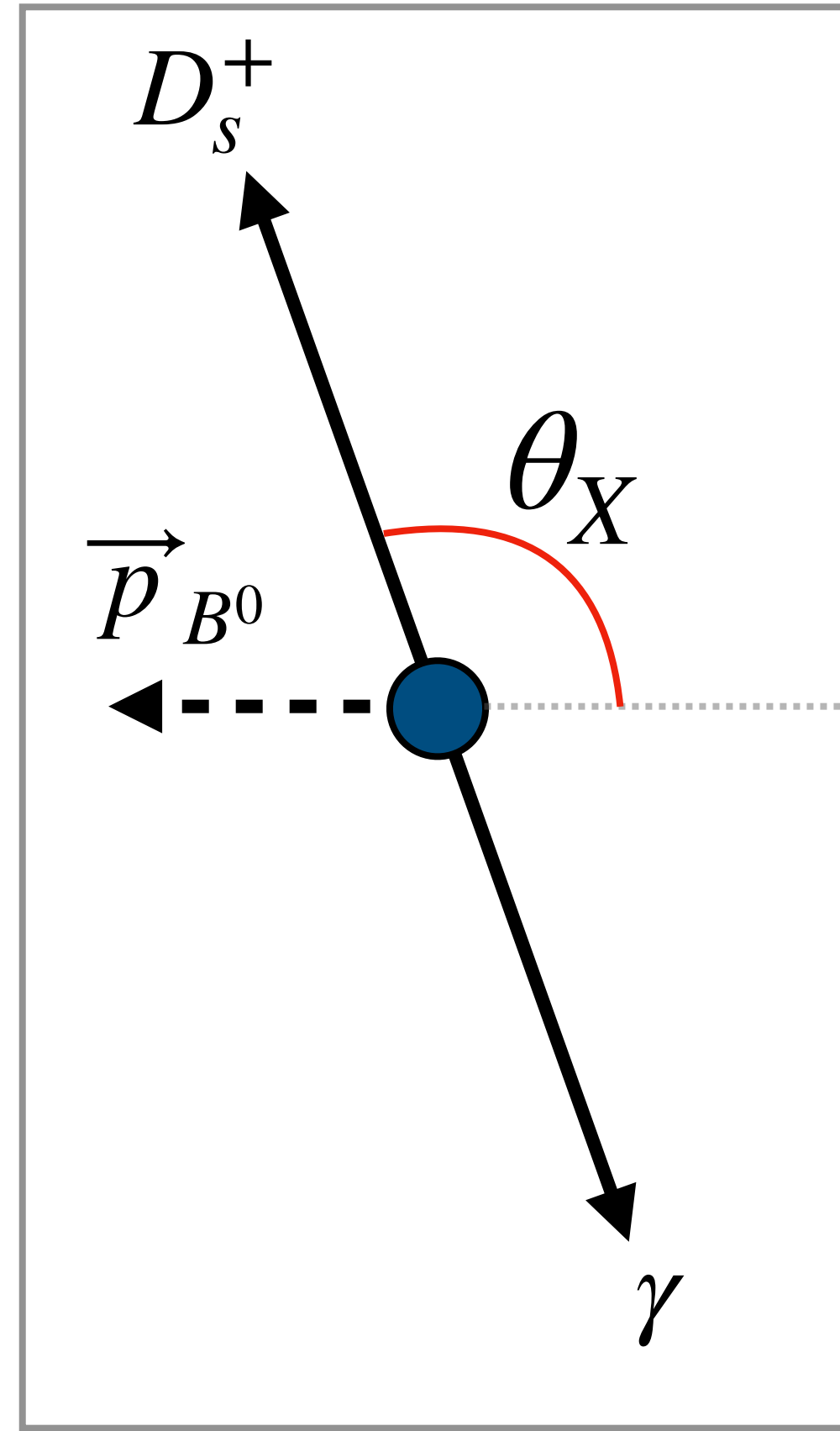
D_s^{*+} rest frame
