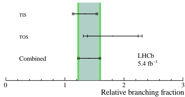
Figure 1: Measured relative branching fraction for the TOS and TIS samples and the combined result. The inner error bars represent statistical uncertainties and the outer error bars represent the total uncertainties.
