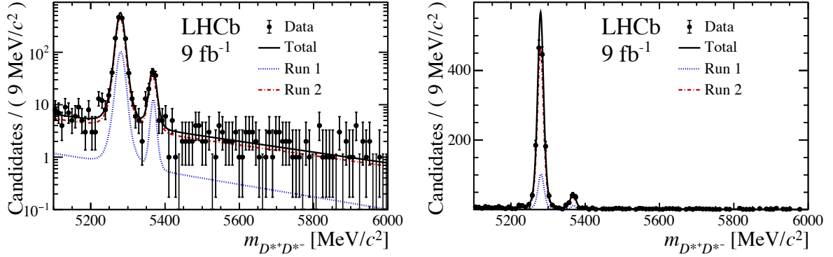
Figure 3: Distributions of the D^{*+}D^{*-} mass combining both data-taking periods with (left) logarithmic and (right) linear y axes. In addition to the total fit result (solid black), each of the individual components are shown: the (dotted blue) Run 1 and the (dash-dotted red) Run 2 data-taking periods.
